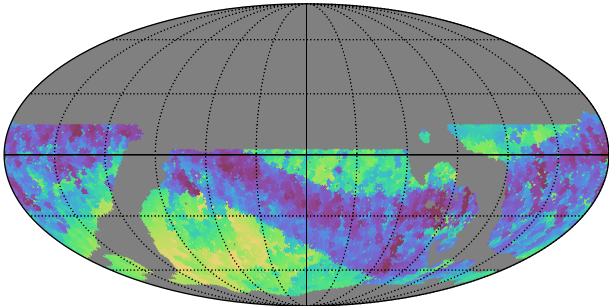
roll_pause_mjdp365_v3.4_10yrs WFD i band: Min skyBrightness
