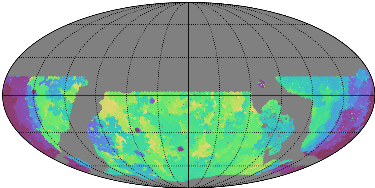
roll_pause_mjdp365_v3.4_10yrs WFD g band: Min skyBrightness
