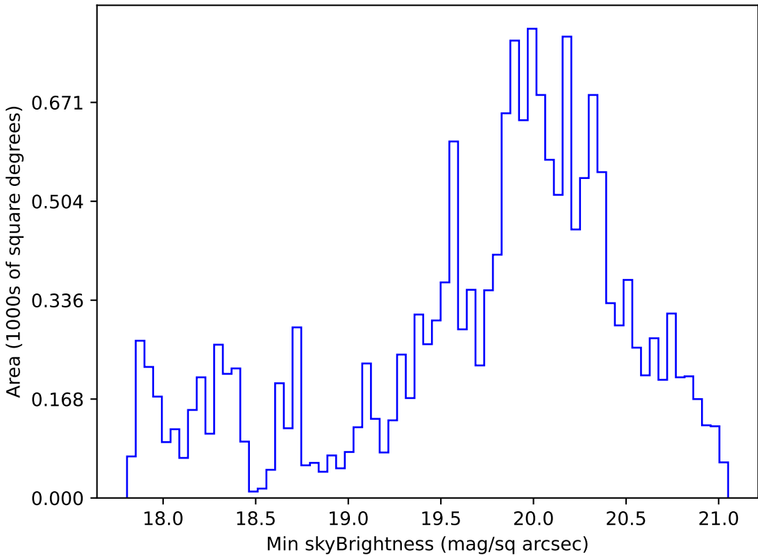
roll_pause_mjdp365_v3.4_10yrs WFD g band: Min skyBrightness
