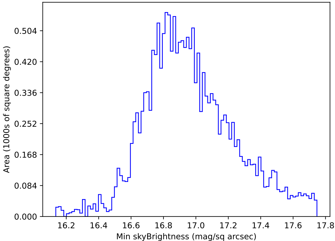
roll_pause_mjdp365_v3.4_10yrs WFD all bands: Min skyBrightness
