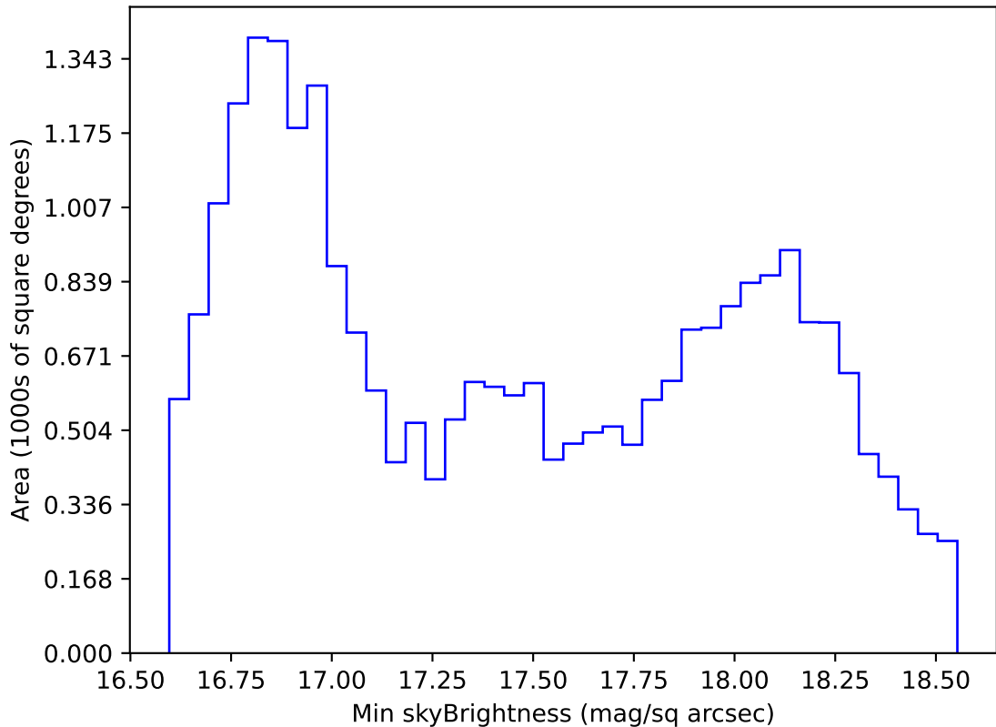
roll_pause_mjdp365_v3.4_10yrs All sky z band: Min skyBrightness
