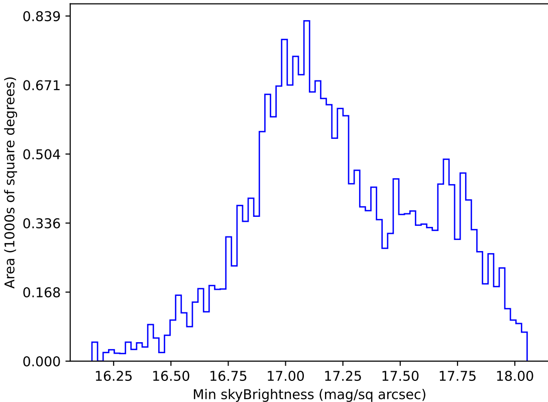
roll_pause_mjdp365_v3.4_10yrs All sky y band: Min skyBrightness
