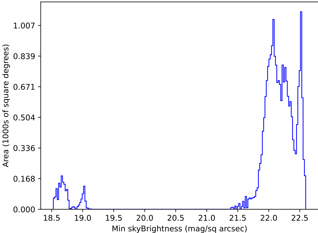
roll_pause_mjdp365_v3.4_10yrs All sky u band: Min skyBrightness
