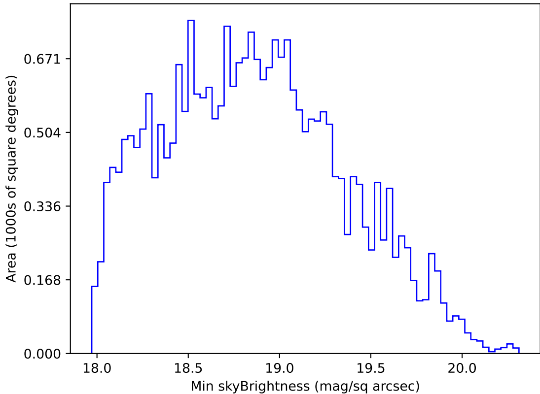
roll_pause_mjdp365_v3.4_10yrs All sky r band: Min skyBrightness
