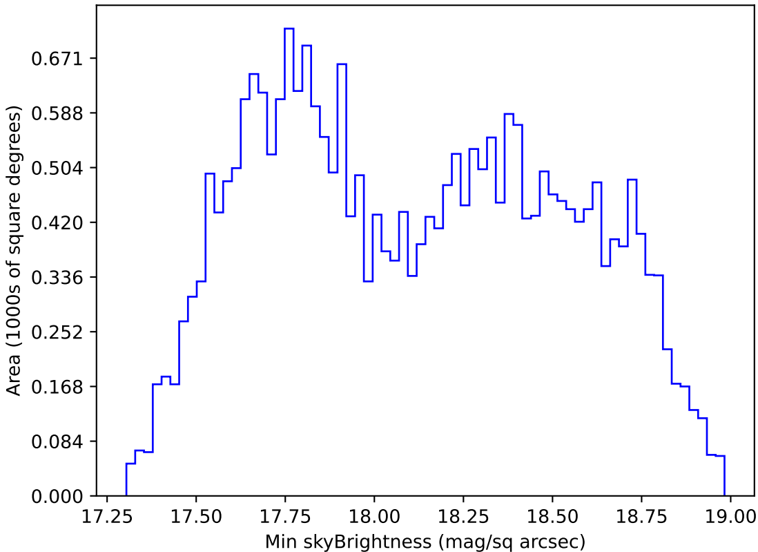
roll_pause_mjdp365_v3.4_10yrs All sky i band: Min skyBrightness
