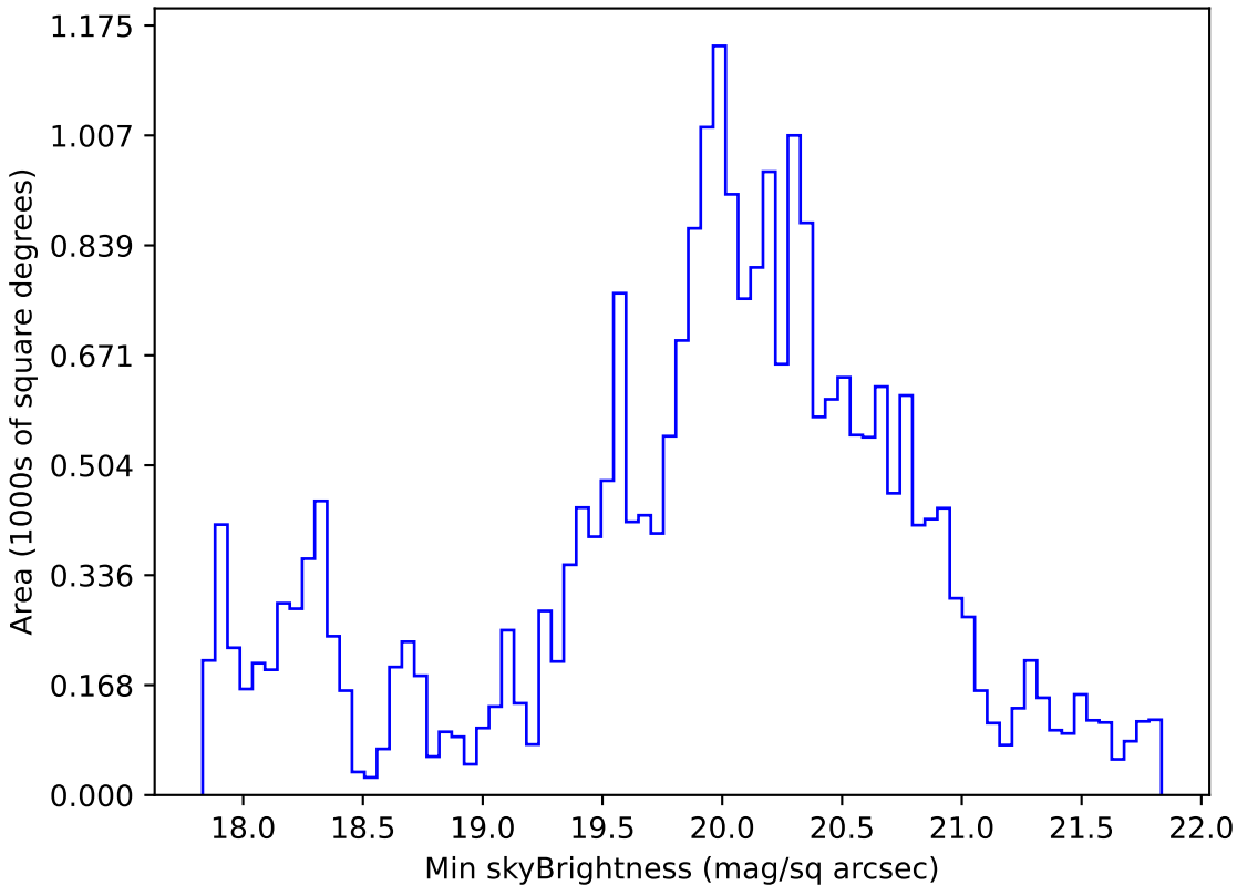
roll_pause_mjdp365_v3.4_10yrs All sky g band: Min skyBrightness
