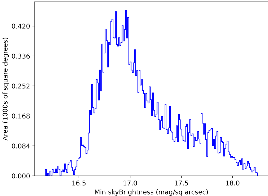
roll_pause_mjdp365_v3.4_10yrs All sky all bands: Min skyBrightness
