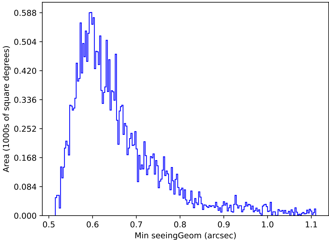
roll_pause_mjdp365_v3.4_10yrs Yr 1 z band: Min seeingGeom
