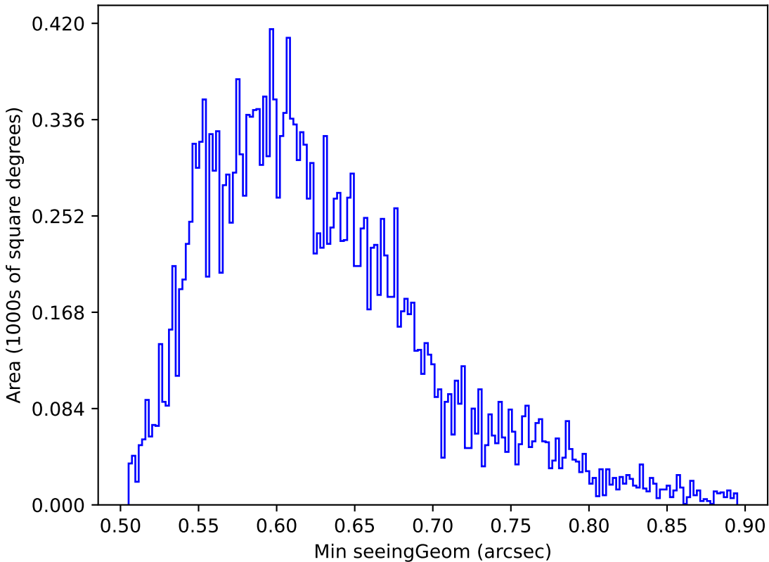
roll_pause_mjdp365_v3.4_10yrs Yr 1 y band: Min seeingGeom
