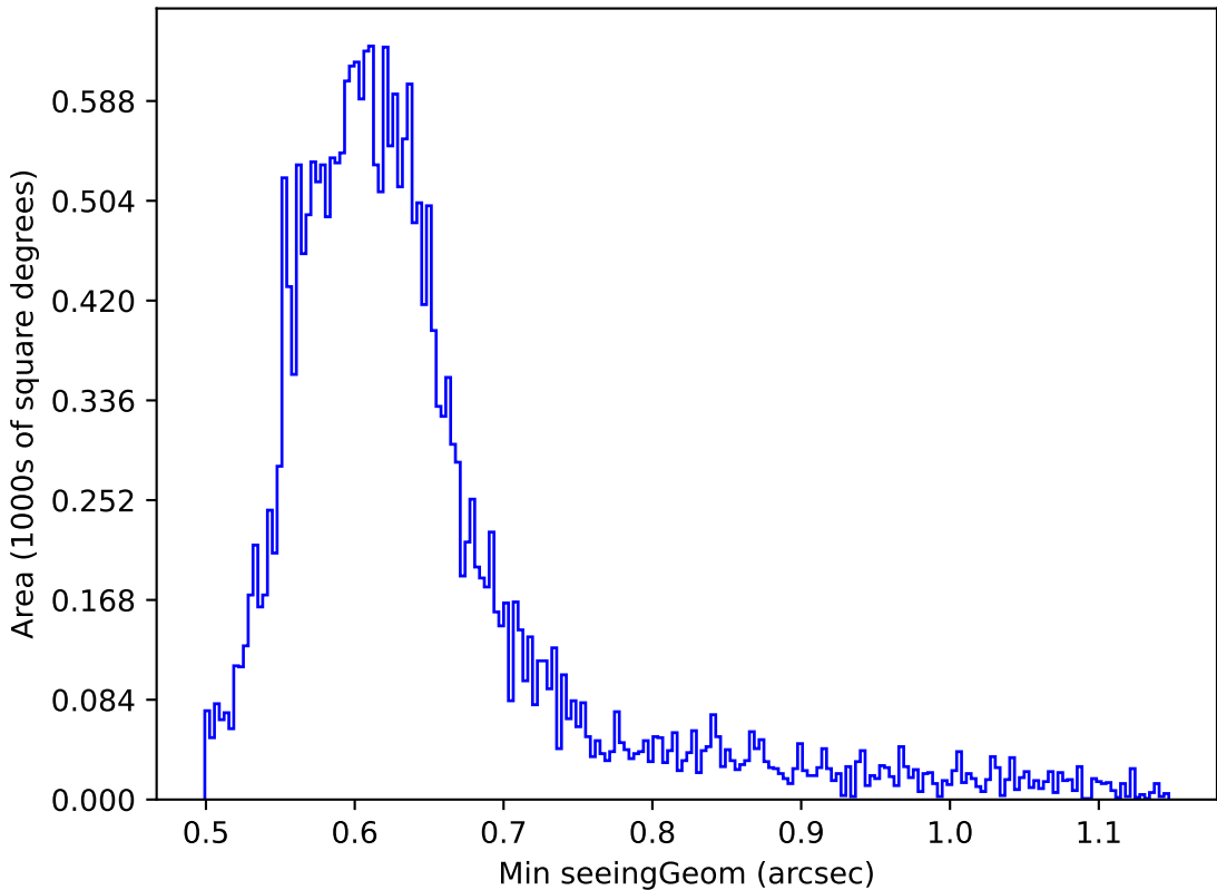
roll_pause_mjdp365_v3.4_10yrs Yr 1 r band: Min seeingGeom
