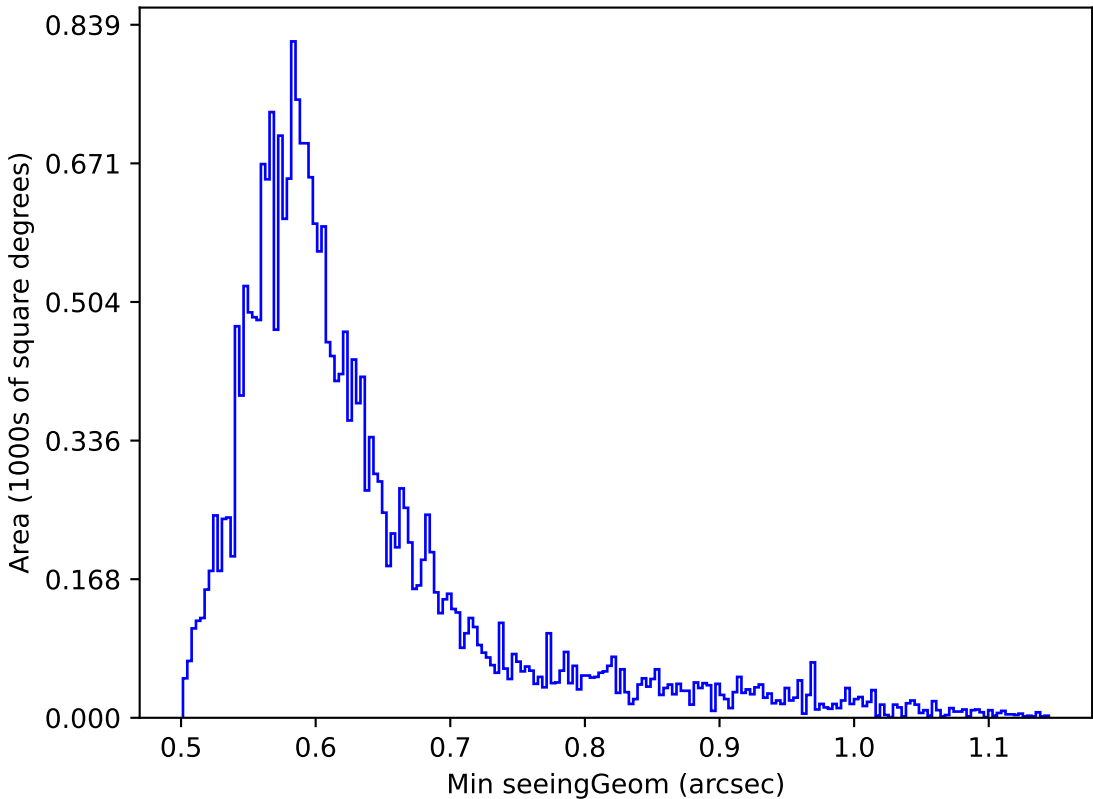
roll_pause_mjdp365_v3.4_10yrs Yr 1 i band: Min seeingGeom
