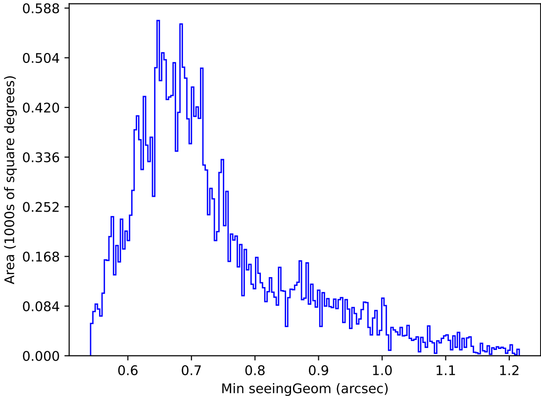
roll_pause_mjdp365_v3.4_10yrs Yr 1 g band: Min seeingGeom
