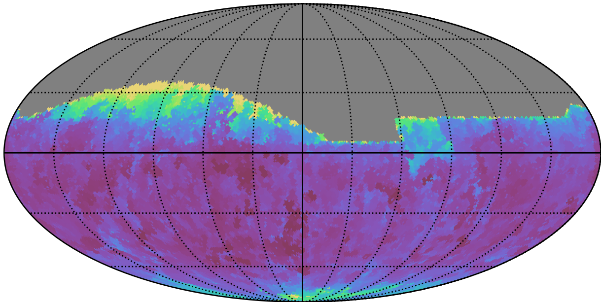
roll_pause_mjdp365_v3.4_10yrs Yr 1 all bands: Min seeingGeom
