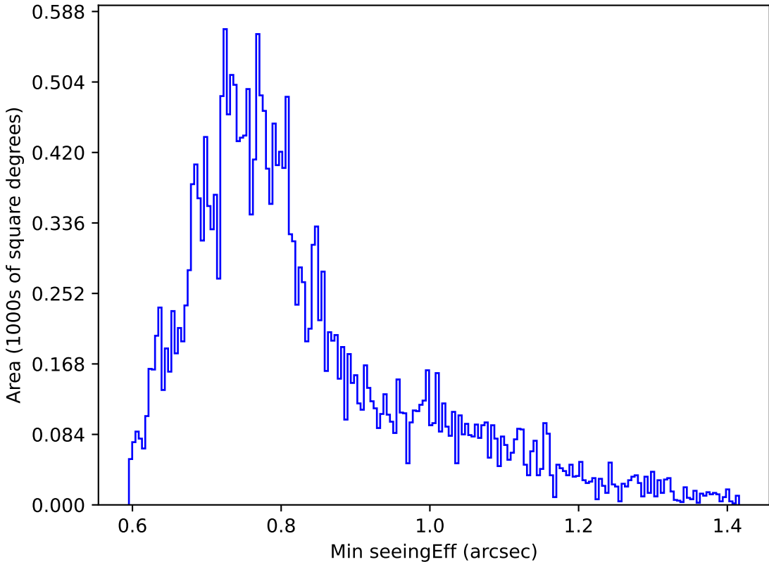
roll_pause_mjdp365_v3.4_10yrs Yr 1 g band: Min seeingEff
