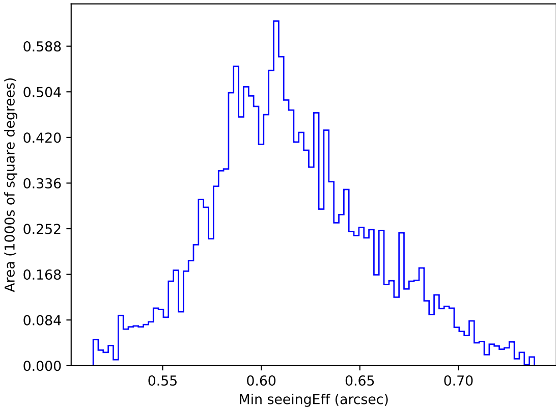
roll_pause_mjdp365_v3.4_10yrs WFD z band: Min seeingEff
