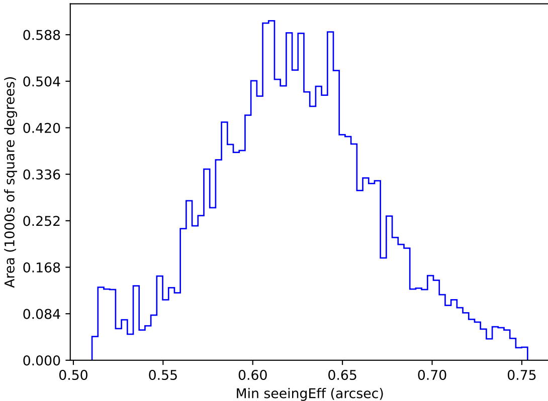
roll_pause_mjdp365_v3.4_10yrs WFD y band: Min seeingEff
