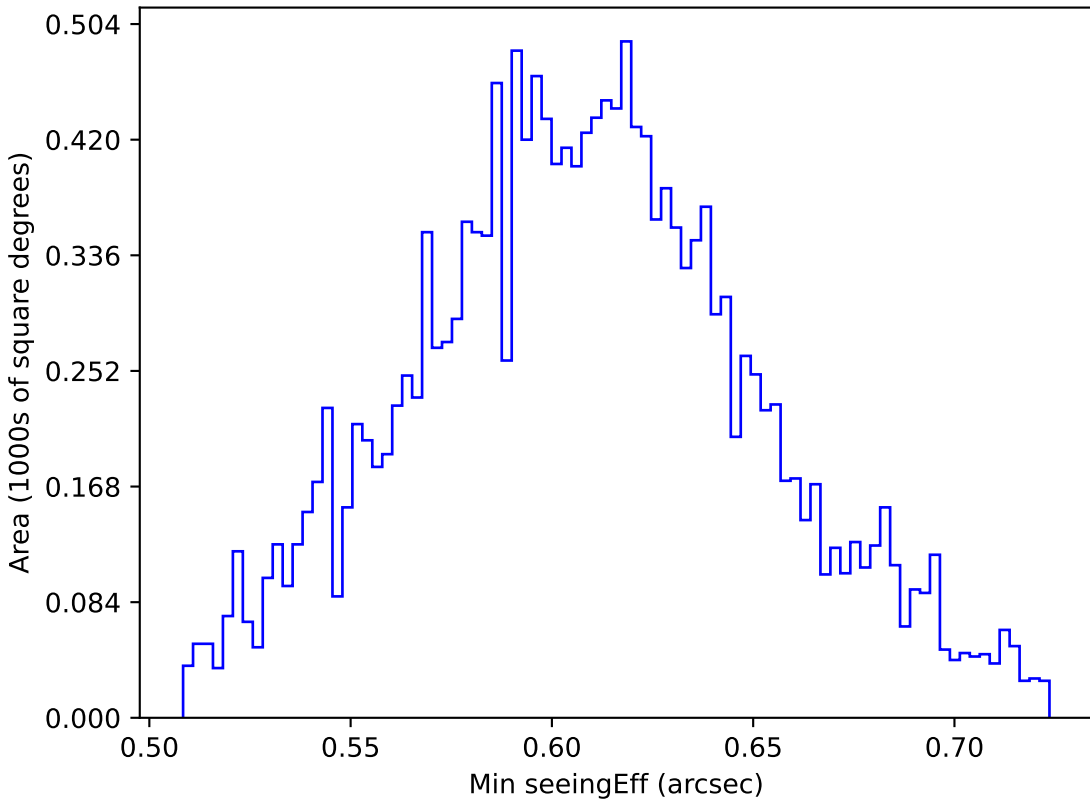
roll_pause_mjdp365_v3.4_10yrs WFD r band: Min seeingEff
