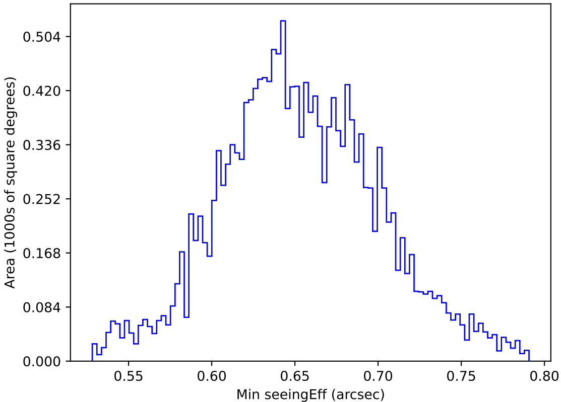
roll_pause_mjdp365_v3.4_10yrs WFD g band: Min seeingEff
