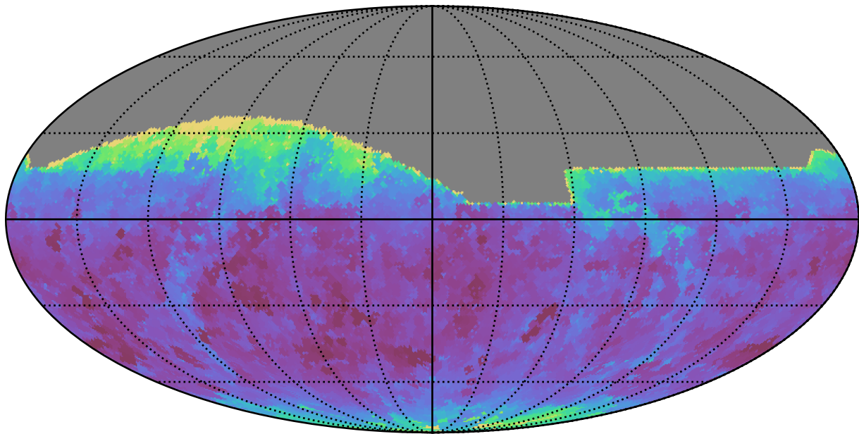
roll_pause_mjdp365_v3.4_10yrs All sky z band: Min seeingEff
