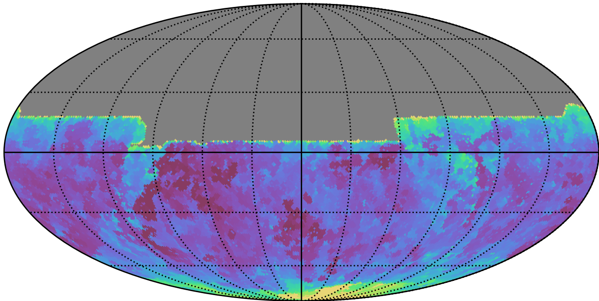
roll_pause_mjdp365_v3.4_10yrs All sky y band: Min seeingEff
