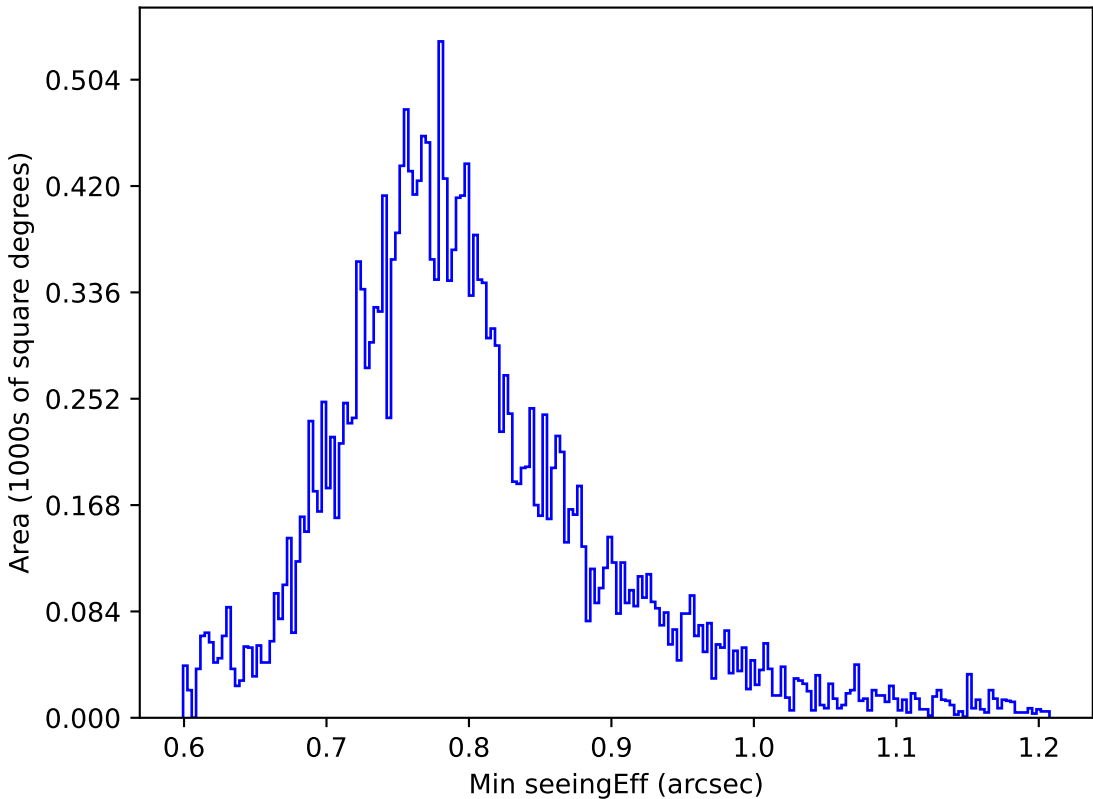
roll_pause_mjdp365_v3.4_10yrs All sky u band: Min seeingEff
