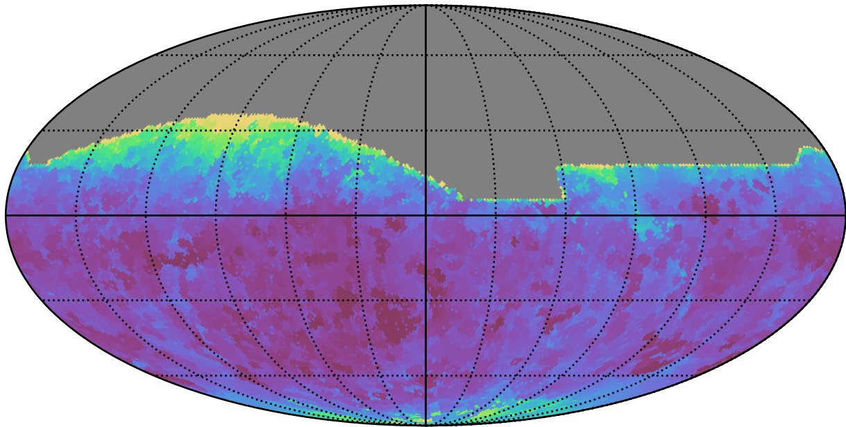
roll_pause_mjdp365_v3.4_10yrs All sky i band: Min seeingEff
