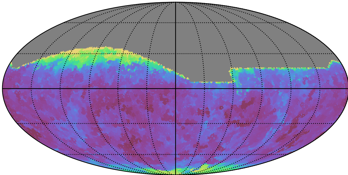
roll_pause_mjdp365_v3.4_10yrs All sky g band: Min seeingEff
