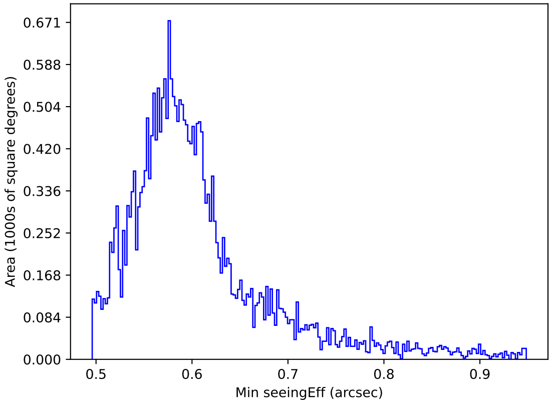
roll_pause_mjdp365_v3.4_10yrs All sky all bands: Min seeingEff
