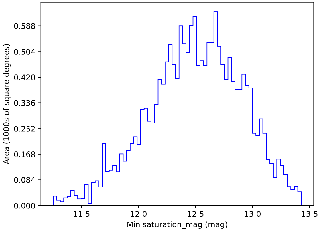
roll_pause_mjdp365_v3.4_10yrs WFD r band: Min saturation_mag
