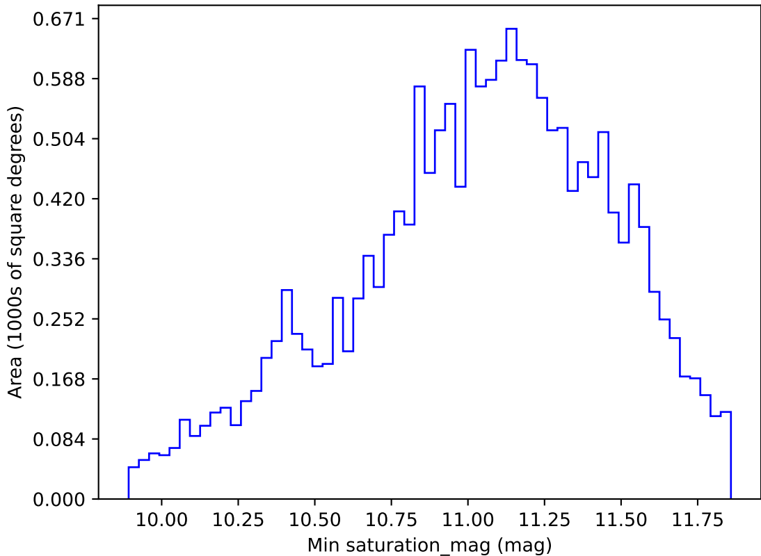
roll_pause_mjdp365_v3.4_10yrs WFD all bands: Min saturation_mag
