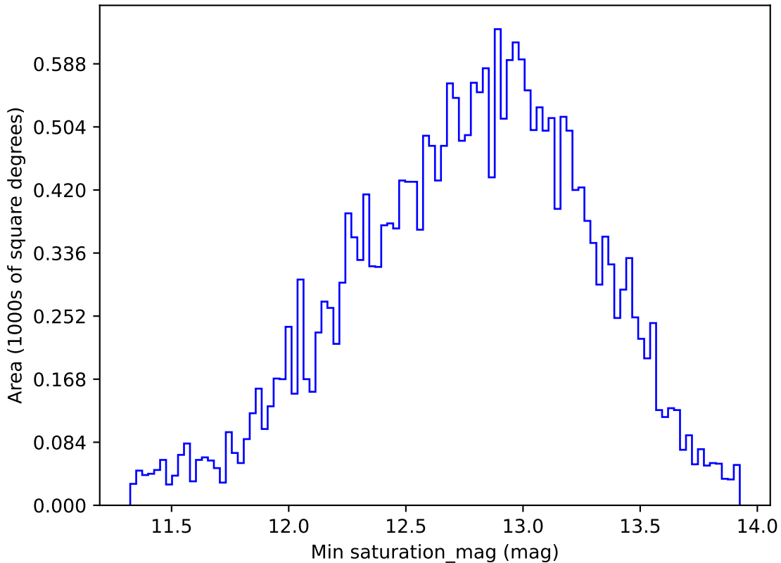
roll_pause_mjdp365_v3.4_10yrs All sky g band: Min saturation_mag
