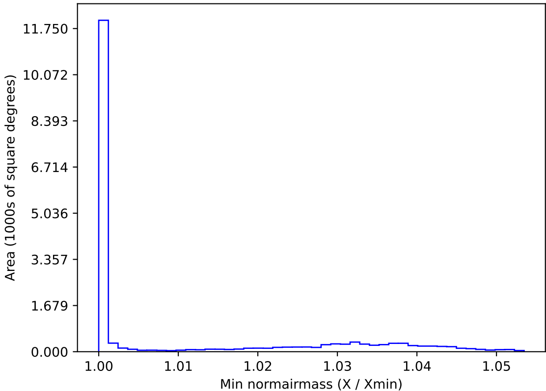
roll_pause_mjdp365_v3.4_10yrs WFD u band: Min normairmass
