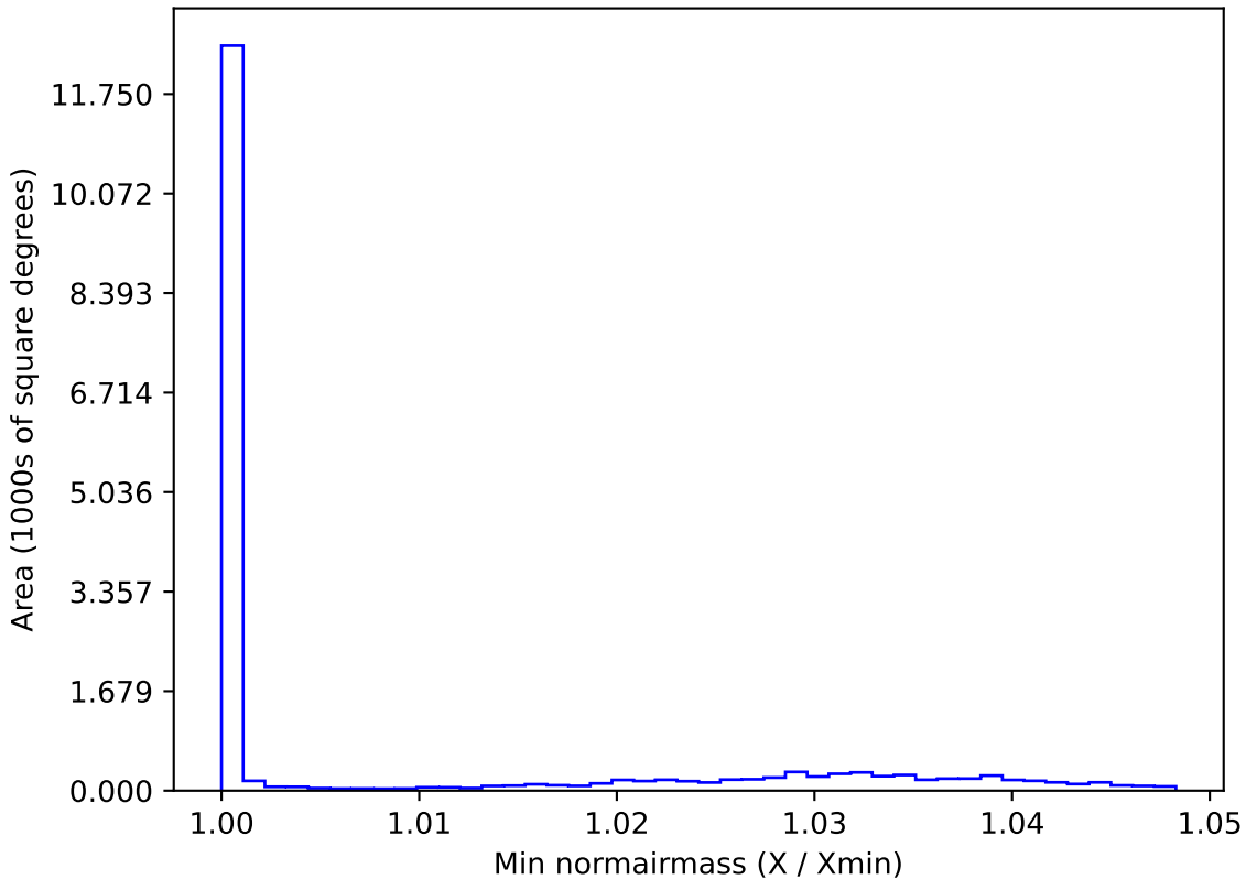
roll_pause_mjdp365_v3.4_10yrs WFD g band: Min normairmass
