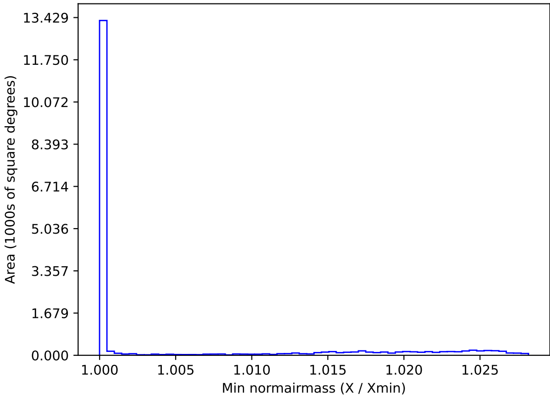
roll_pause_mjdp365_v3.4_10yrs WFD all bands: Min normairmass
