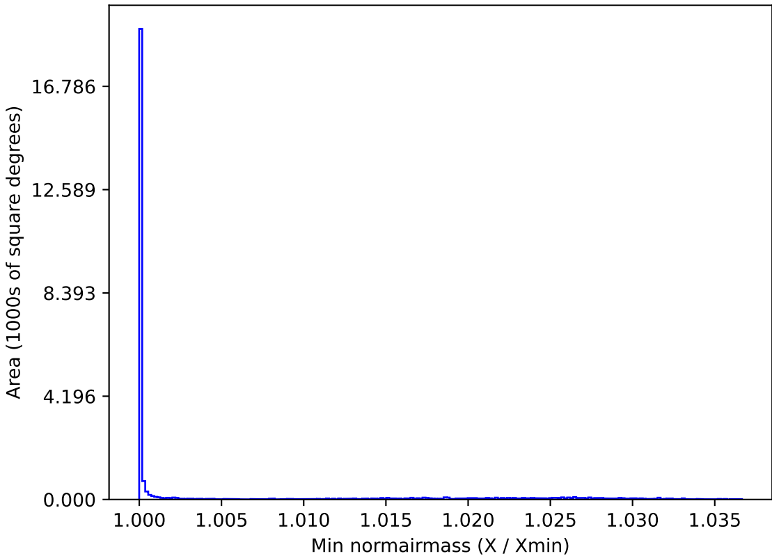
roll_pause_mjdp365_v3.4_10yrs All sky r band: Min normairmass
