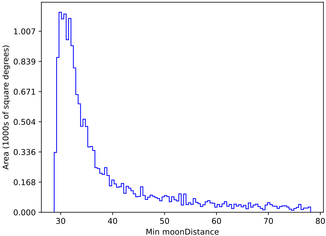
roll_pause_mjdp365_v3.4_10yrs WFD r band: Min moonDistance
