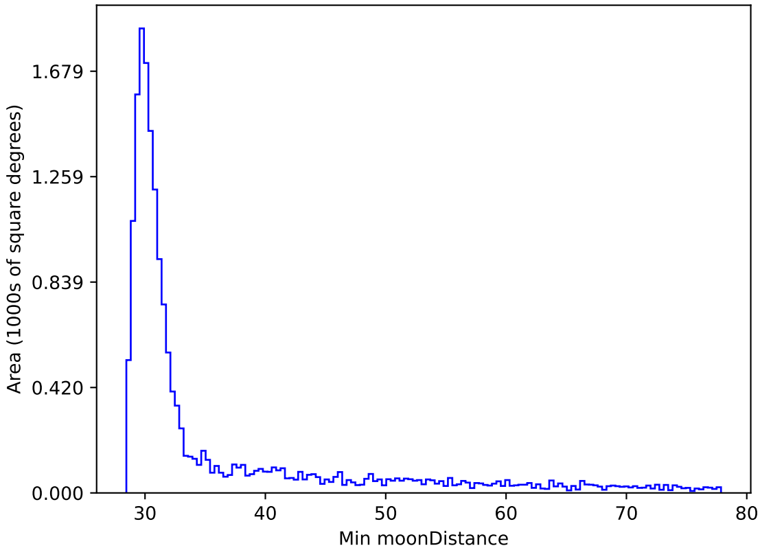
roll_pause_mjdp365_v3.4_10yrs WFD i band: Min moonDistance
