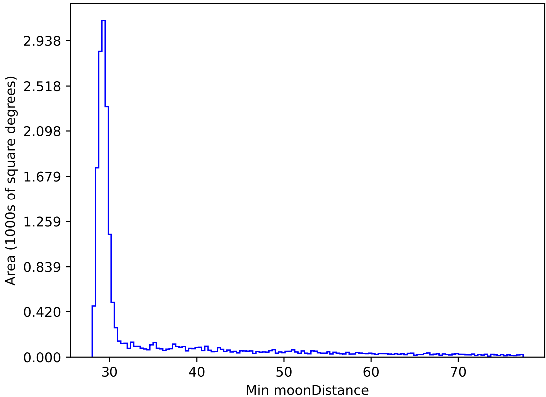
roll_pause_mjdp365_v3.4_10yrs WFD all bands: Min moonDistance
