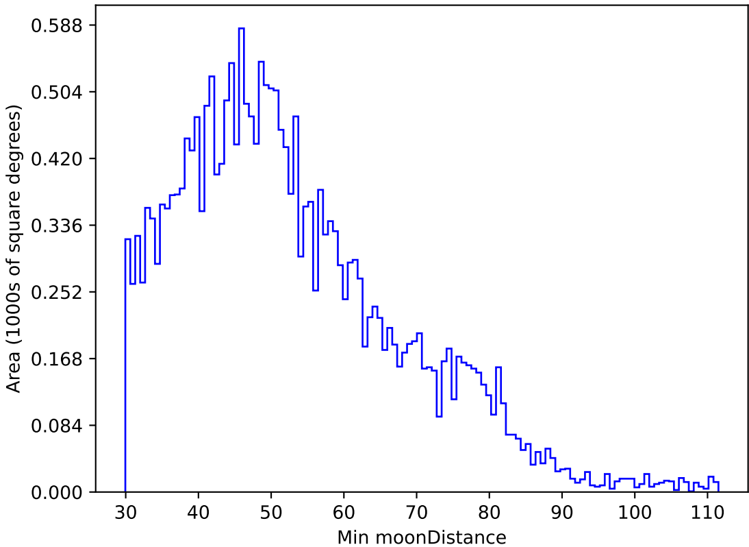
roll_pause_mjdp365_v3.4_10yrs All sky u band: Min moonDistance
