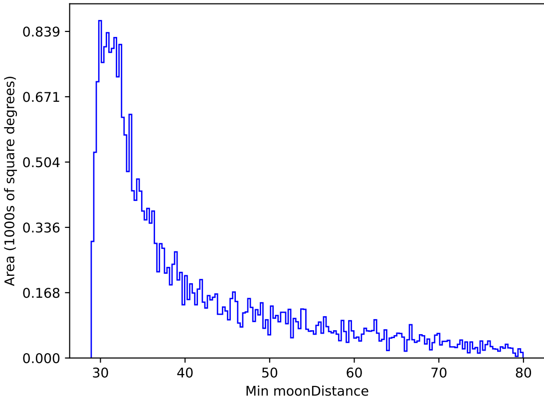
roll_pause_mjdp365_v3.4_10yrs All sky r band: Min moonDistance
