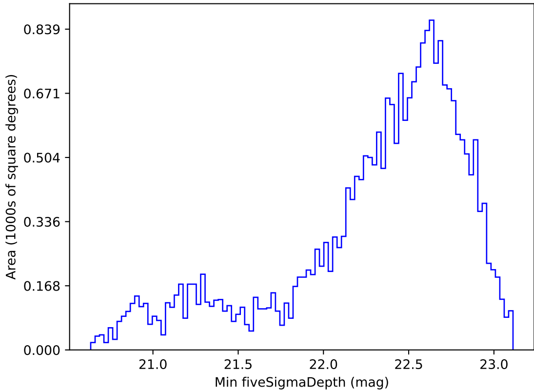
roll_pause_mjdp365_v3.4_10yrs Yr 1 z band: Min fiveSigmaDepth
