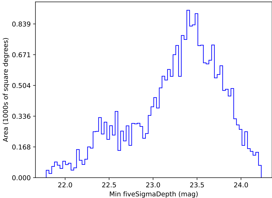
roll_pause_mjdp365_v3.4_10yrs Yr 1 r band: Min fiveSigmaDepth
