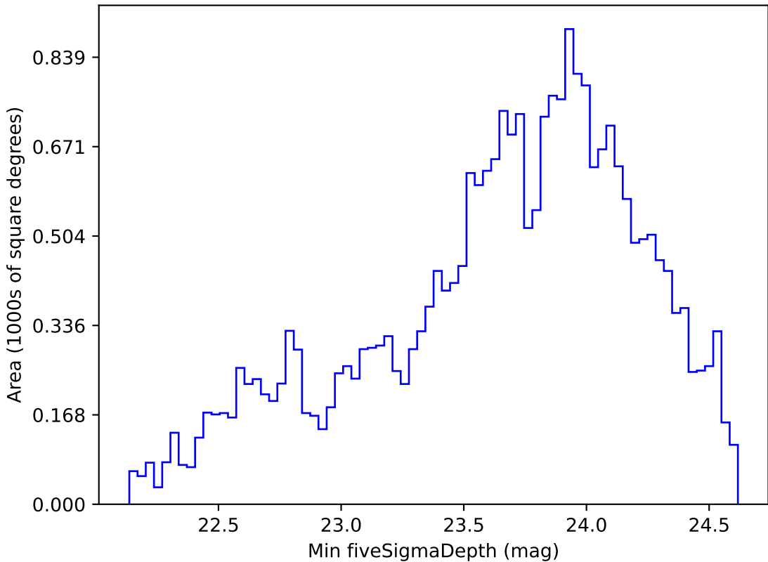
roll_pause_mjdp365_v3.4_10yrs Yr 1 g band: Min fiveSigmaDepth
