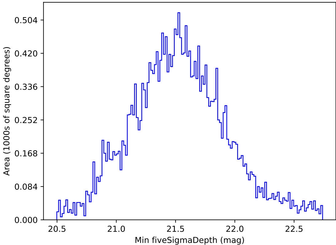
roll_pause_mjdp365_v3.4_10yrs Yr 1 all bands: Min fiveSigmaDepth
