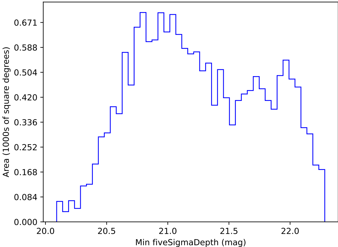
roll_pause_mjdp365_v3.4_10yrs WFD z band: Min fiveSigmaDepth
