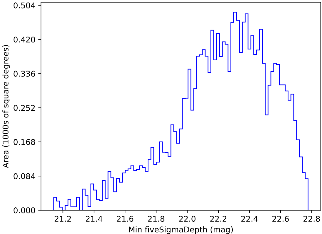
roll_pause_mjdp365_v3.4_10yrs WFD u band: Min fiveSigmaDepth
