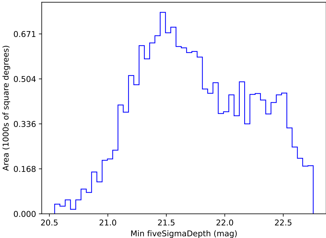
roll_pause_mjdp365_v3.4_10yrs WFD i band: Min fiveSigmaDepth
