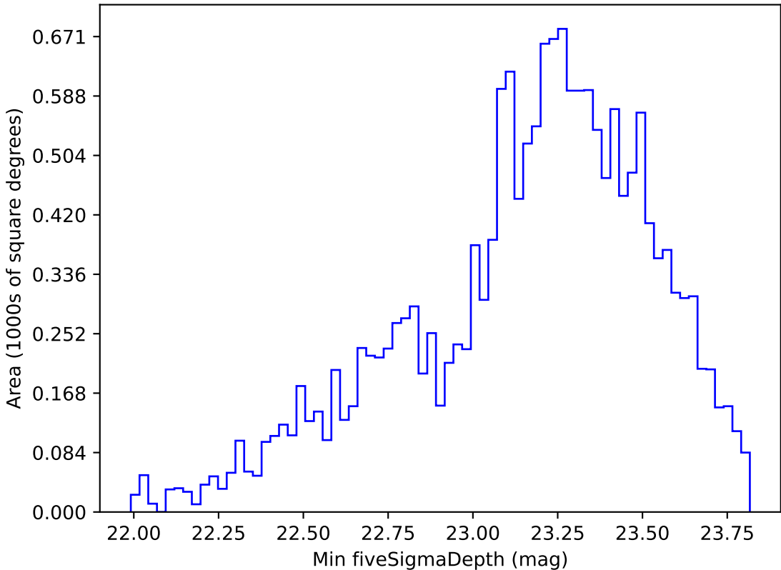
roll_pause_mjdp365_v3.4_10yrs WFD g band: Min fiveSigmaDepth
