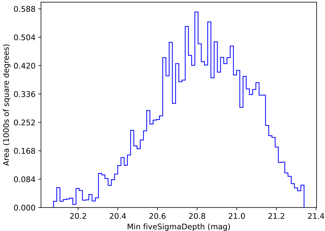
roll_pause_mjdp365_v3.4_10yrs WFD all bands: Min fiveSigmaDepth
