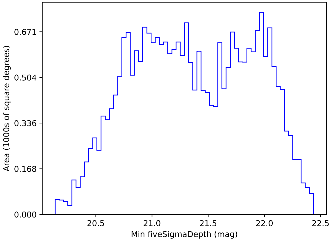
roll_pause_mjdp365_v3.4_10yrs All sky z band: Min fiveSigmaDepth
